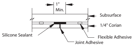
Hard Seam
