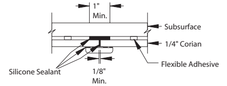
Batten-Covered Seam
