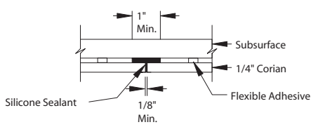
Silicone Seam
