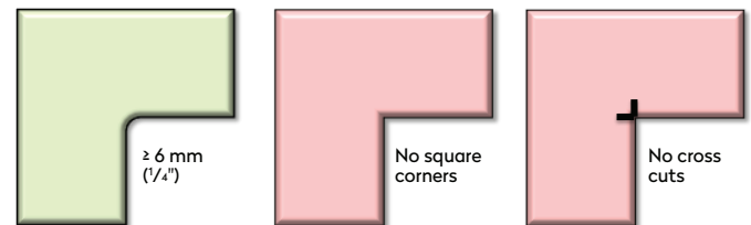
Figure E-2: Inside Corner Requirements
