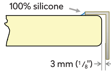
Figure I-2: Gap for Top Mount Sink
